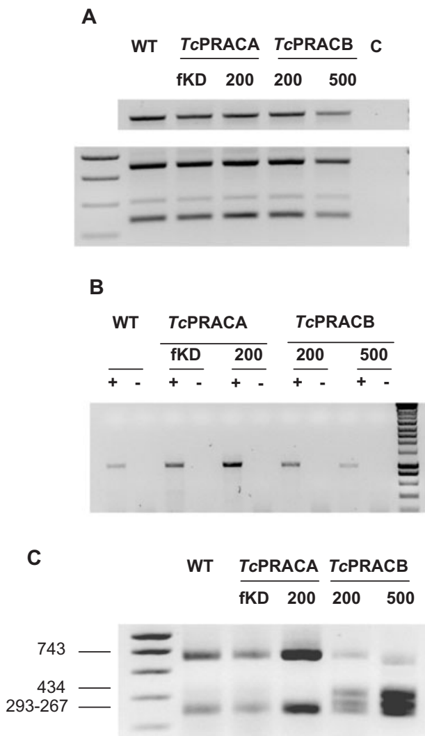
Fig. 3. RT-PCR analysis of polyA RNA from TcPRACA and TcPRACB transgenic parasites. A. PCR amplification of genomic DNA with TcPRAC Hi/RAB-specific primers from wild-type (WT) and transgenic parasites for TcPRACA and TcPRACB genes (top), and GsuI enzyme restriction analysis of resultant fragments (bottom), fractionated on a 1.5% agarose gel containing ethidium bromide; C, internal negative control. B. mRNA expression of TcPRAC in WT or transfected parasites shown by electrophoresis of gene fragments obtained by oligo(dT)-primed reverse transcription from total RNA extracted from equivalent parasite numbers, followed by PCR amplification using the sequences of the mini-exon (spliced leader, SLp) and RAB primers. First-strand cDNA reactions were performed in the presence (+) or absence (-) of reverse transcriptase, to exclude the possibility of further PCR amplification of fragments due to genomic DNA contamination. C. RT-PCR amplified fragments were digested with GsuI and analysed on a 1.5% agarose gel containing ethidium bromide. Molecular sizes (kb) of the fragments are indicated.
