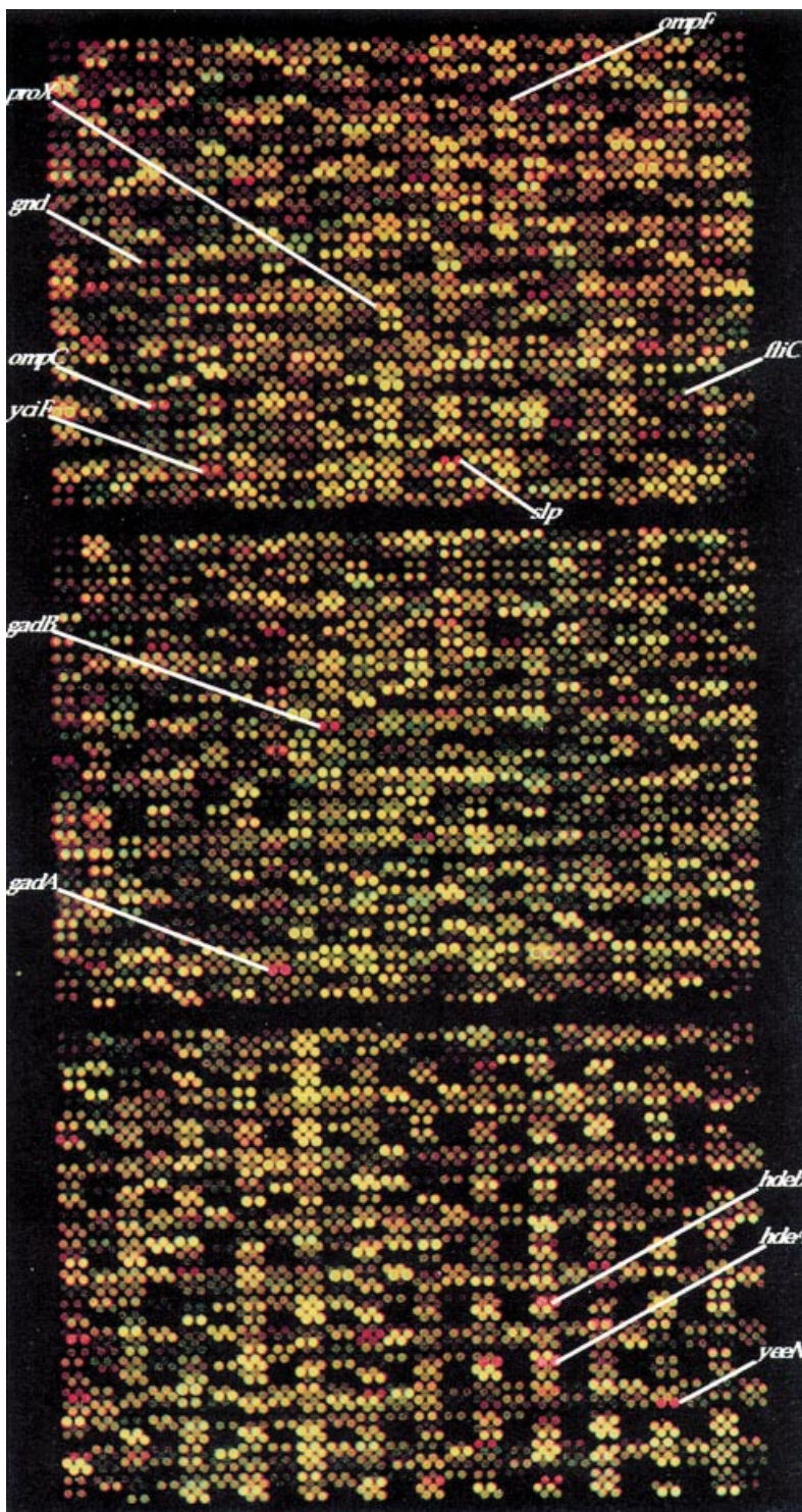
Fig. 3. Overlay of DNA arrays hybridized with wild-type or hns mutant cDNA. Variations in gene expression were measured with DNA arrays containing the 4290 open reading frames (ORFs) of the E. coli genome hybridized with cDNA probes generated from RNA extracted from wild-type and hns BE1410 mutant strains. Macroarrays were scanned as described in Experimental procedures , and the ADOBE PHOTOSHOP F1-4.0 software was used to produce the overlay of representative macroarrays. The macroarray hybridized with the hns mutant cDNA probes was coloured red and that with the wild-type cDNA probes was coloured green. Genes whose expression was not modified in H-NS-deficient and wild-type strains are coloured yellow, and those induced or repressed in the hns mutant are coloured red or green respectively. Genes whose product showed an altered accumulation level between wild-type and hns strains (Fig. 1) are indicated by an arrow and named.
