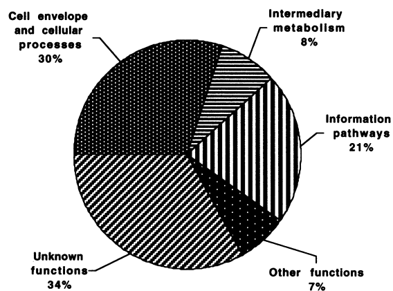
Fig. 4. Functional classification of H-NS-regulated genes identified by expression profiling on DNA arrays. Genes that showed a differential expression between wild-type and mutant strain ( P -value \leq 0.05 ) were classified according to their function (Moszer, 1998).
