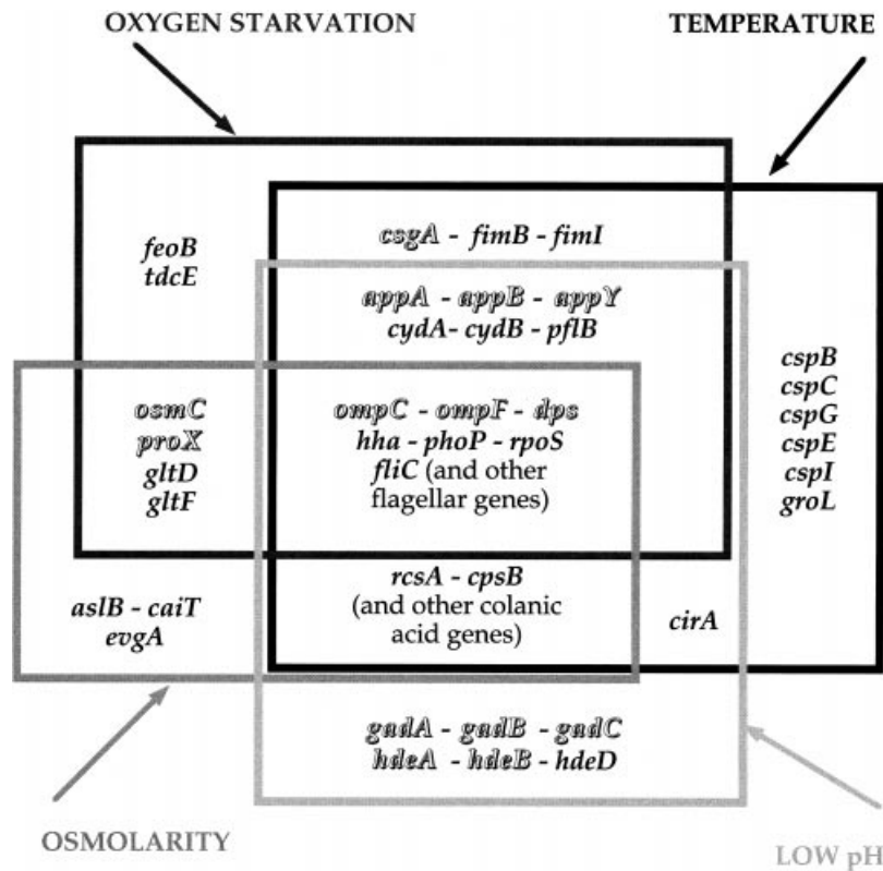
Fig. 6. H-NS regulon genes and their regulation by environmental parameters. Genes of known function that were found to be either directly or indirectly controlled by H-NS on two-dimensional gels (Fig. 1) and/or macroarrays (Table 1) were clustered according to the conditions known to modulate their expression. Rectangles represent genes belonging to oxygen, temperature, osmolarity and pH regulon respectively. Genes written in shaded are those identified previously as RpoS-regulated genes.
