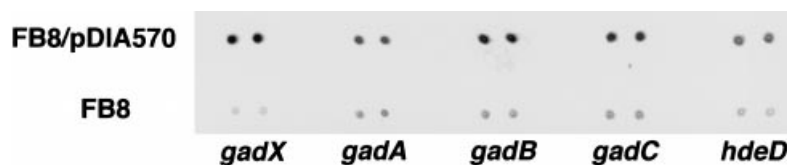
Fig. 5. Effect of gadX overexpression on pH-regulated genes. DNA fragments were amplified by PCR using primers specific for the 5' and 3' ends of the corresponding nucleotide sequence (Sigma-GenoSys Biotechnologies) and spotted in duplicate using a Q Pix arrayer (Genetix). Wild-type FB8 strains in the presence or not of pDIA570 overexpressing gadX were grown to A_{600} = 0.5 in minimal medium, pH 5.5, supplemented with 0.4% glucose and 0.012% glutamate. RNAs were extracted by a rapid procedure (I. Guilloard, unpublished), and cDNA probes were prepared with random hexamer primers (F. Hommais, unpublished). After hybridization, the results were quantified as described in Experimental procedures .
