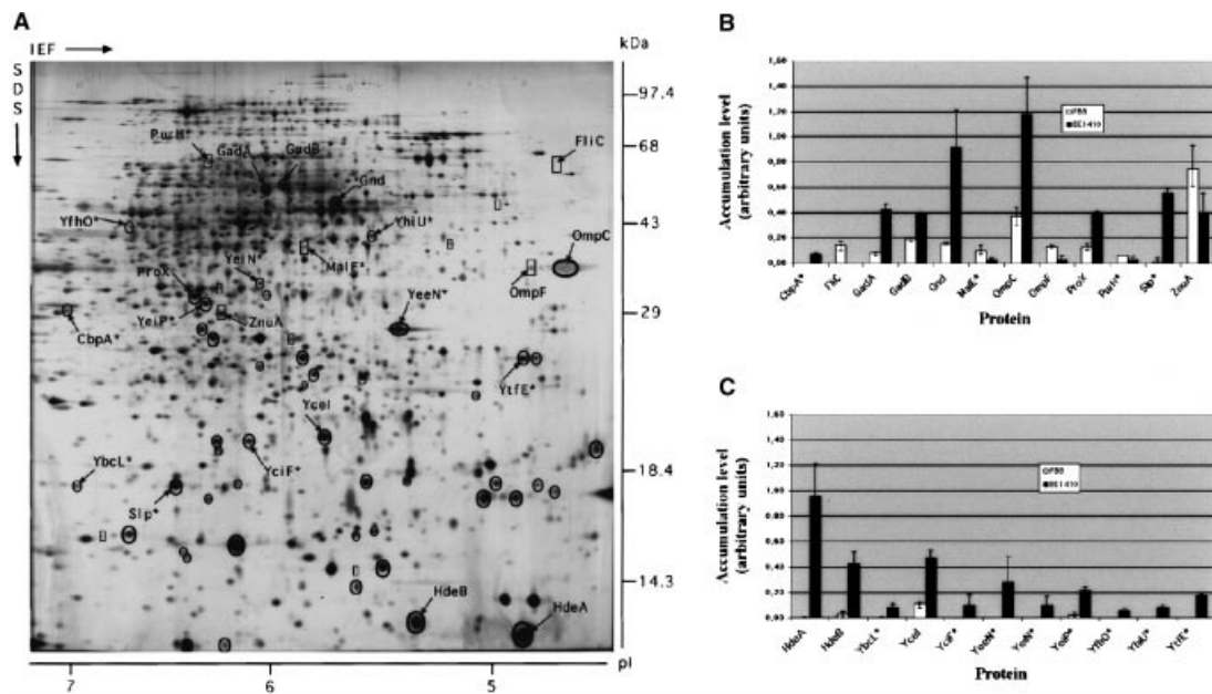
Fig. 1. Two-dimensional silver-stained map of the H-NS-deficient strain, BE1410, and comparative analysis of the level of accumulated proteins in the wild-type and hns mutant strains. Two-dimensional gel electrophoresis (A) was carried out as described in Experimental procedures . The 49 proteins represented by a circle and the 11 proteins represented by a rectangle correspond to polypeptides whose accumulation level was increased and decreased, respectively, in all experiments by at least a factor of two in BE1410 compared with the FB8 wild-type strain. The 23 identified spots are named and indicated by an arrow; those characterized by mass spectrometry are indicated by *. Protein levels are expressed as percentage volume, which corresponds to the percentage ratio between the volume of a single spot and the total volume of all spots present in a gel. The accumulation level of proteins with known function (B) and of putative or unknown function (C) in the wild-type strain (□) and in the hns mutant (■) was quantified using the MELANIE II software (Bio-Rad). The data are the mean values \pm standard deviations of four independent experiments. The BLASTP program and the Prosite patterns database were used to compare the amino acid sequences of proteins with putative or unknown function (C) with the updated non-redundant databases. HdeA (P26604) has been proposed to have a chaperone-like function in extremely acidic conditions in pathogenic enteric bacteria. YeiN, YeeN and YtfE were similar to proteins of unknown function from Thermotoga maritima , B. subtilis and Haemophilus influenzae , respectively. YbcL belongs to the UPF0098 protein family, which comprises proteins of unknown function from Mycobacterium tuberculosis and Archeoglobus fulgidus . The YeiP (P33028) sequence was similar to elongation factors from various bacteria and contained the elongation factor P signature (PS01275); YfhO (P39171) was similar to pyridoxal phosphate enzymes and contained the corresponding signature (class V pyridoxal phosphate attachment site, PS00595). YhiU (P37636) was similar to the acriflavin resistance protein from E. coli and contained the prokaryotic membrane lipoprotein lipid attachment site (PS00013).
