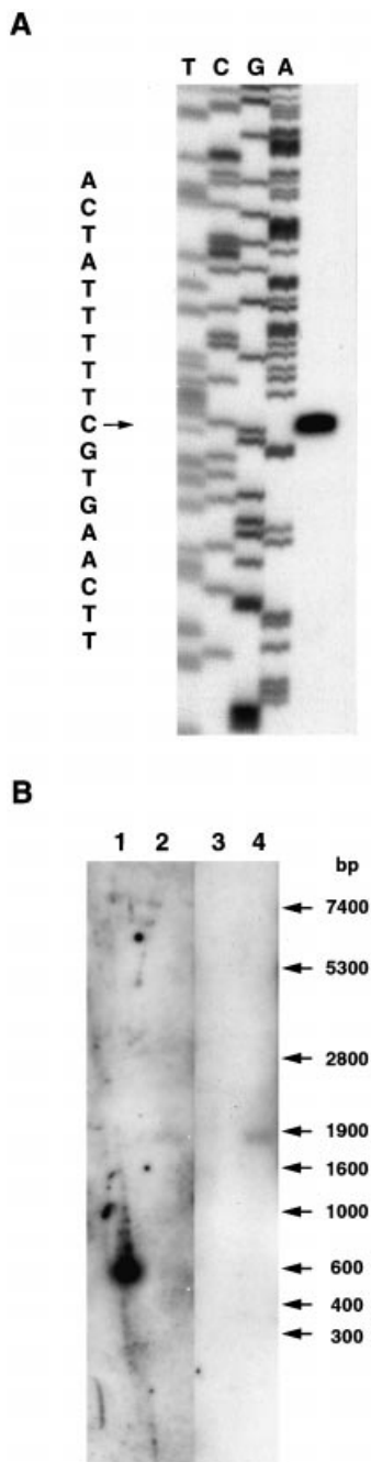
Fig. 5. Identification of the speD promoter by primer extension and of the speD transcripts by Northern blotting.
