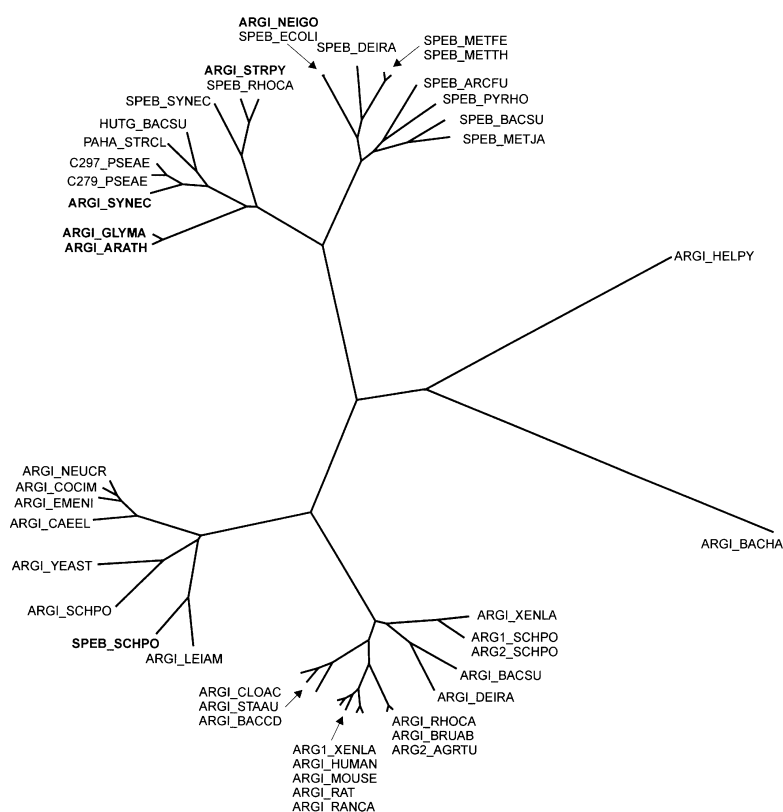
Fig. 3. Gap-tree of ureohydrolases and related enzymes, calculated by factorial analysis of the lengths of the insertions in the multiple alignments (roman numeral in Fig. 1). This is not a phylogenetic reconstruction, but a distance tree based on the conservation of the position and length of probable loops in the three-dimensional structure of the proteins.
