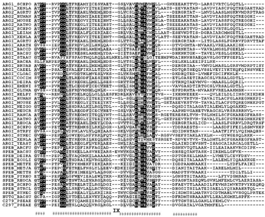
Fig. 1. Multiple alignment of 50 sequences of ureohydrolases and related enzymes, as obtained from CLUSTAL W and DIALIGN, manually edited in the regions containing many non-contiguous gaps. The highly divergent N and C termini have been removed. Identical and similar residues in more than 75% of the sequences are drawn on black and shaded backgrounds, respectively. Those residues that were kept for the phylogenetic reconstructions are labelled '#', the excluded parts corresponding to regions where CLUSTAL W and DIALIGN gave highly different alignments. The roman numerals point to the regions that were used for building the 'gap tree' (see Results and Fig. 3). The arrows point to the residues involved in the binding of manganese ions. In this figure and the following ones, the names of the proteins follow the SWISS-PROT convention: ARG1 and SPEB indicate proteins that are noted as arginases and agmatinases, respectively. The names of the species follow the five-letter code as indicated in Table 1.
